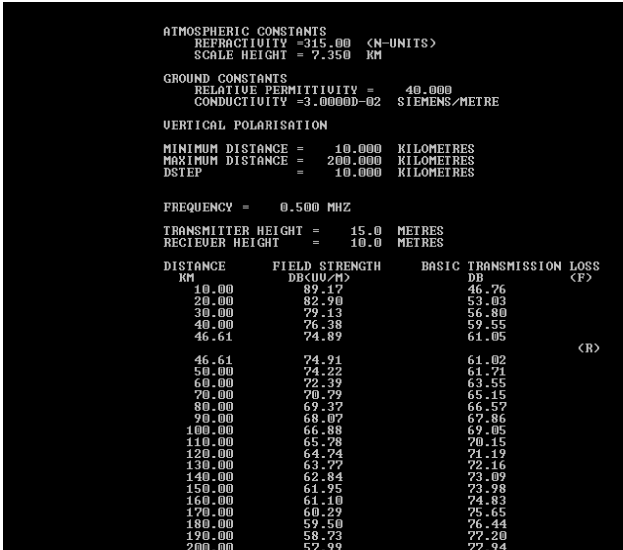
Figure 6: Replication of ITU LF MF Propagation Curve, \sigma = .03S/m , \epsilon = 40 , f\_mhz = .5 mHz
