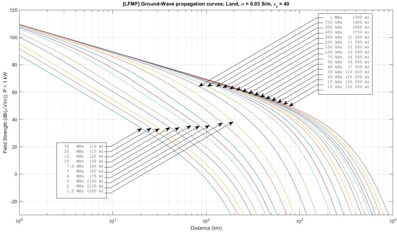
Figure 5: ITU LFMF Propagation Curves, \sigma = .03S/m , \epsilon = 40
